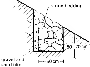
11 Drainage and support of slope base
